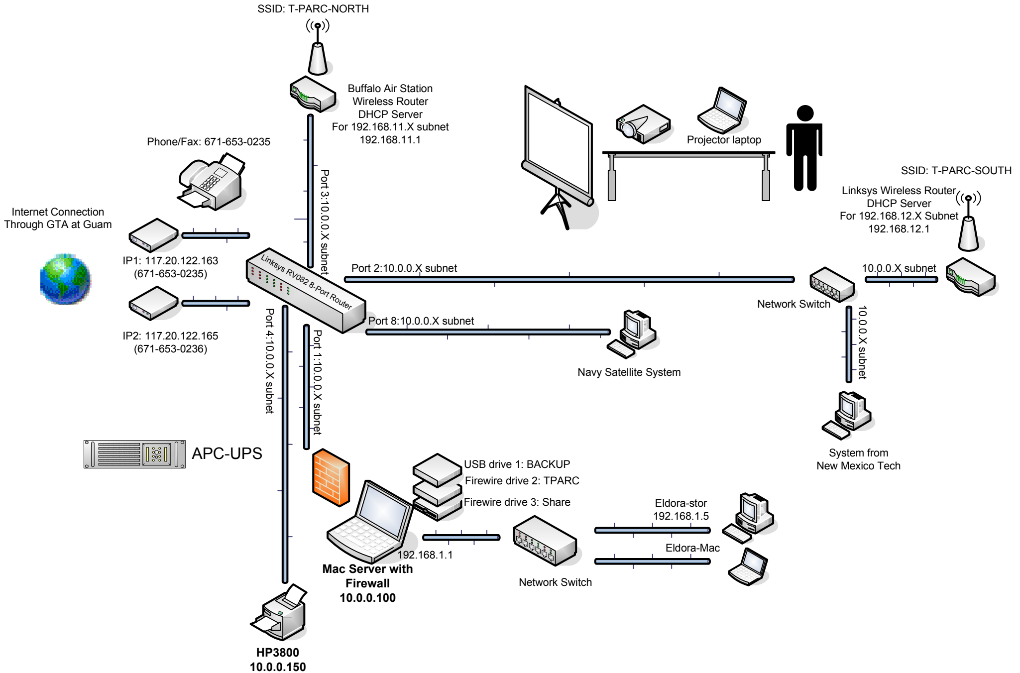
T-PARC Operation Center Network Diagram at CDC of Andersen Airforce Base, Guam Date: 8/1/2008
