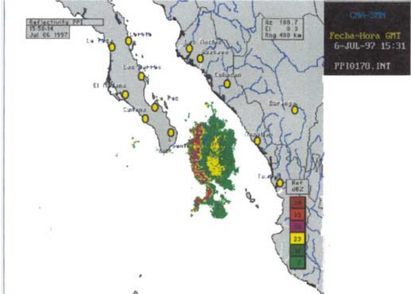
Figure 2. MCS traveling westward from the SMO across GoC (Cabo radar image)
