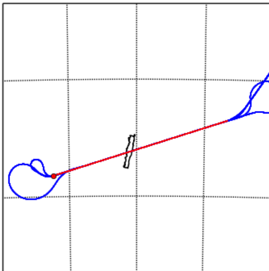
DEEPWAVE RF 23 Flight Track
