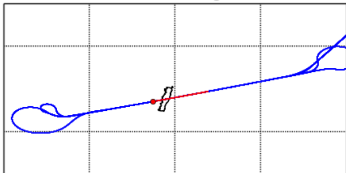
DEEPWAVE RF 23 Flight Track
