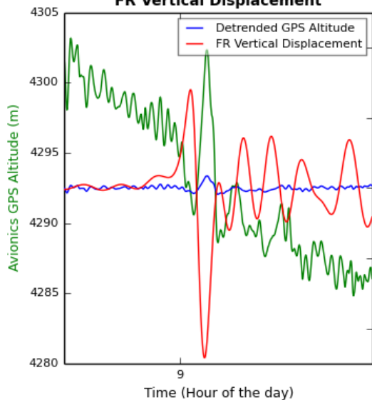
FR Vertical Displacement
