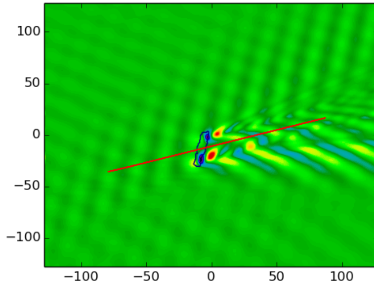
FR simulated W at 4km
