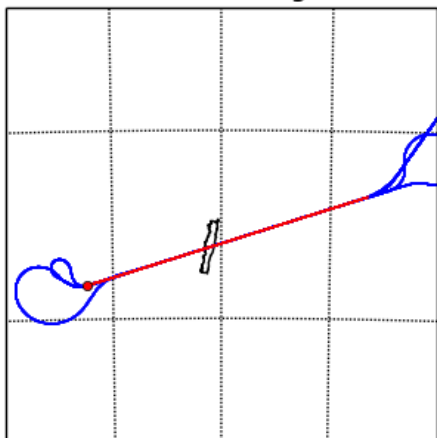
DEEPWAVE RF 23 Flight Track
