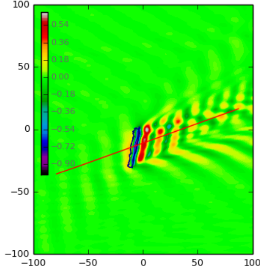
FR Vertical Displacement
