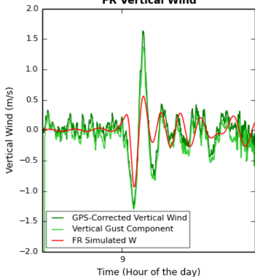
FR Vertical Wind
