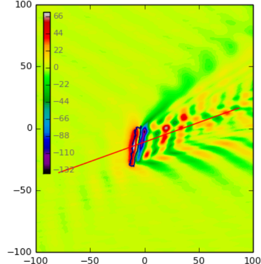
FR Temperature Perturbation
