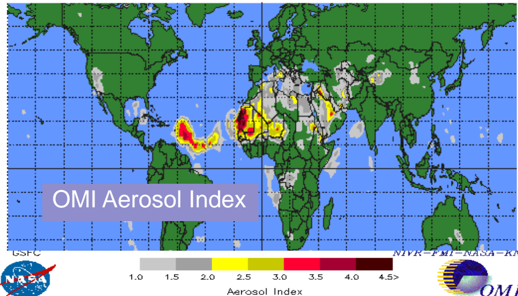
OMI Aerosol Index on June 25, 2007
