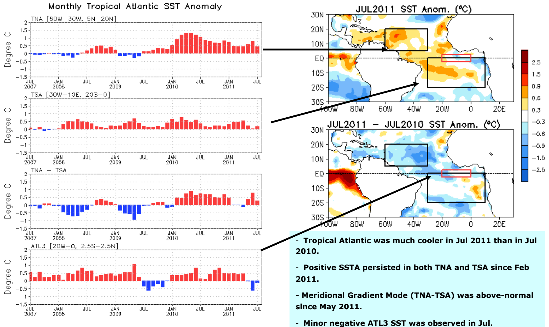
Fig. A1a. Tropical Atlantic Variability region indices, calculated as the area-averaged monthly mean sea surface temperature anomalies (°C) for the TNA [60°W-30°W, 5°N-20°N], TSA [30°W-10°E, 20°S-0], and ATL3 [20°W-0, 2.5°S-2.5°N] regions, and Meridional Gradient Index, defined as differences between TNA and TSA. Data are derived from the NCEP OI SST analysis, and anomalies are departures from the 1971-2000 base period means.
