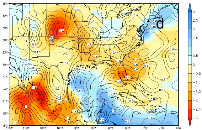
Precipitation ( \text{mmday}^{-1} )
