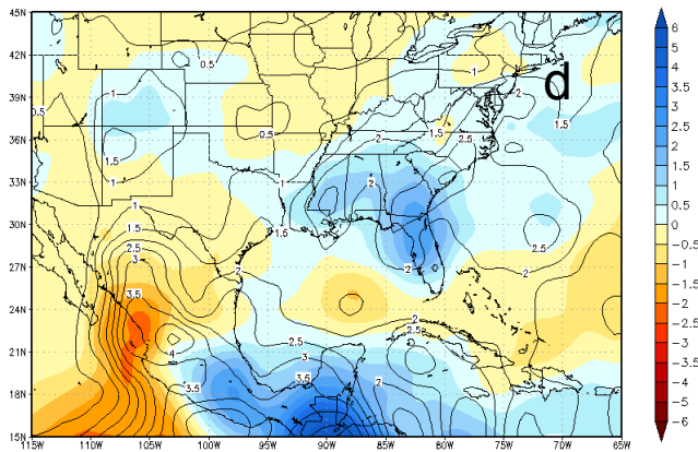
Precipitation ( \text{mmday}^{-1} )
