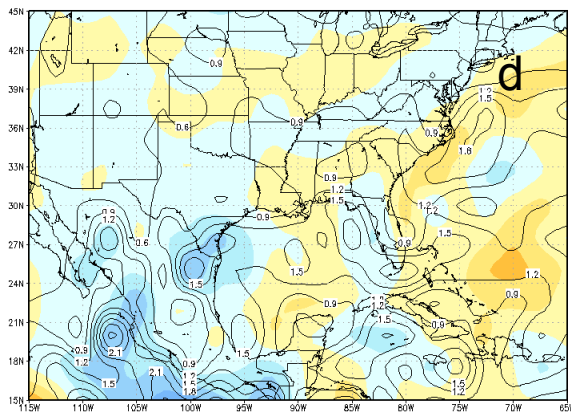
Precipitation ( \text{mmday}^{-1} )
