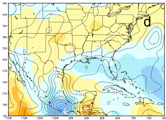
Precipitation ( \text{mmday}^{-1} )
